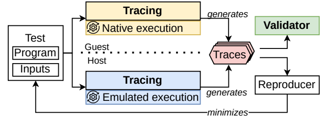
Figure 1. Overview of FOCACCIA’s components: Tracing of native and emulated executions, validation, and reproduction
