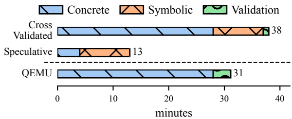
Figure 7. End-to-end runtime comparison for cross-validated, speculative native tracing and QEMU validation for Curl.
