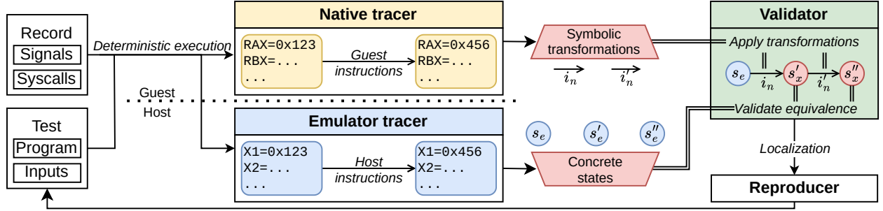
Figure 5. The components in FOCACCIA: native tracer (§ 5.1), emulator tracer (§ 5.2), validator (§ 5.3), and reproducer generator (§ 5.4).
