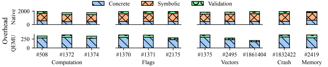
Figure 6. End-to-end overhead breakdown for native tracing and translation validation for QEMU ( \times native execution time).
