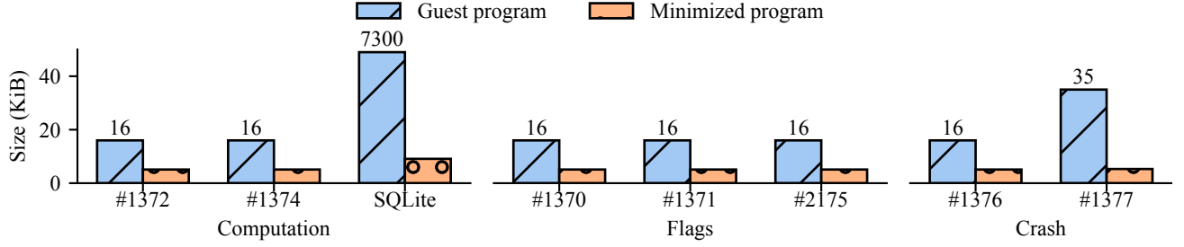
Figure 8. Code size comparison of the guest mistranslated program and the minimized reproducer generated by FOCACCIA.
