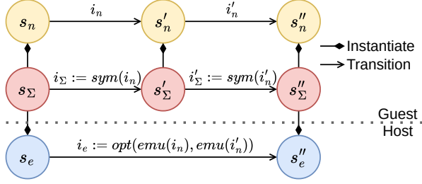
Figure 4. Analogous transitions between native, symbolic, and emulated states. The symbolic state s_\Sigma generalizes over the native state s_n and emulated state s_e .
