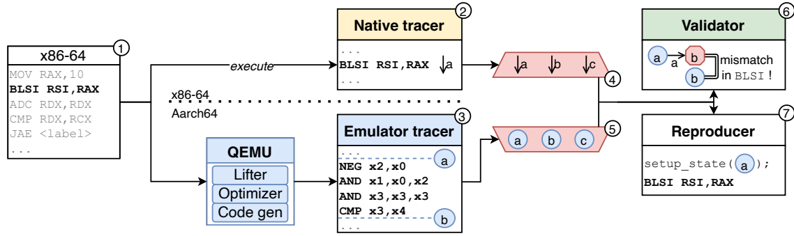
Figure 3. Example of QEMU’s mistranslation of BLSI from x86-64 (guest) to Aarch64 (host), causing #1370.GL [74]
