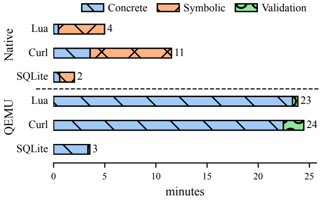
Figure 9. Runtime breakdown for Lua, Curl and SQLite for speculative and selective tracing, and for QEMU validation.
