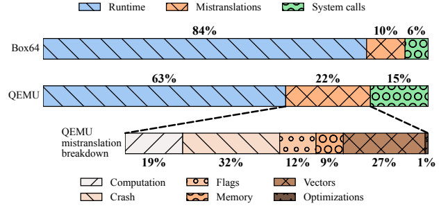
Figure 2. Analysis of user-mode errors in QEMU and Box64.
